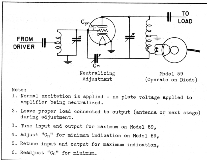
Figure 9 - TRANSMISSION METHOD OF NEUTRALIZATION
